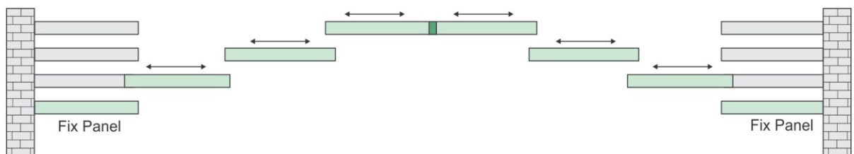
DTS- 3131 (Center opening) 3 Sliding & 1 Fix Panel
