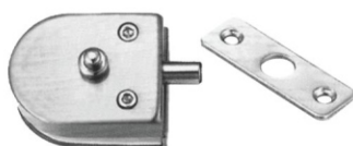
Wall to Glass Lock (Without Cutout) (Inside Push Knob)
